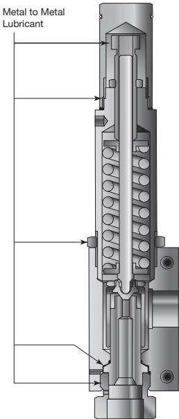
Figure 4 Relief Valve Lubrication Sites
